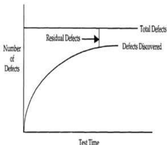
Figure 2 Graphical representation of the weibull and its shape is concave [13]
